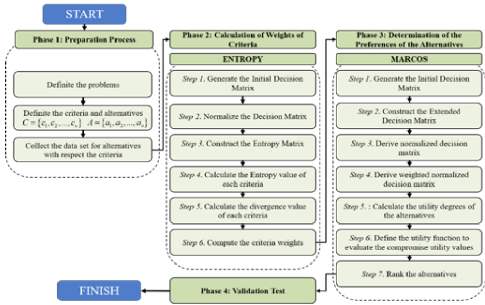
Figure 1. The Basic Algorithm of the proposed integrated MCDM approach
